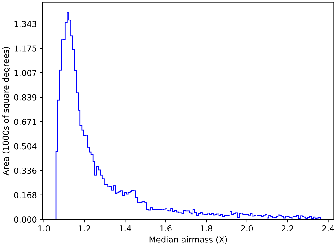
extra_ss_neo2_v3.4_10yrs Yr 1 z band: Median airmass
