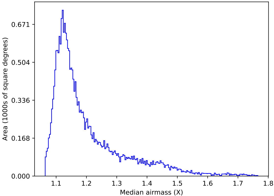
extra_ss_neo2_v3.4_10yrs Yr 1 y band: Median airmass
