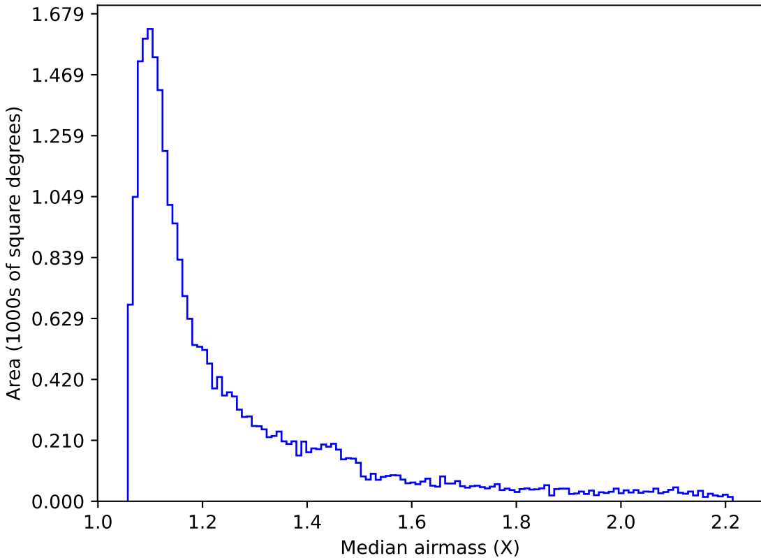
extra_ss_neo2_v3.4_10yrs Yr 1 r band: Median airmass
