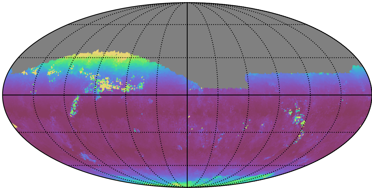
extra_ss_neo2_v3.4_10yrs Yr 1 i band: Median airmass
