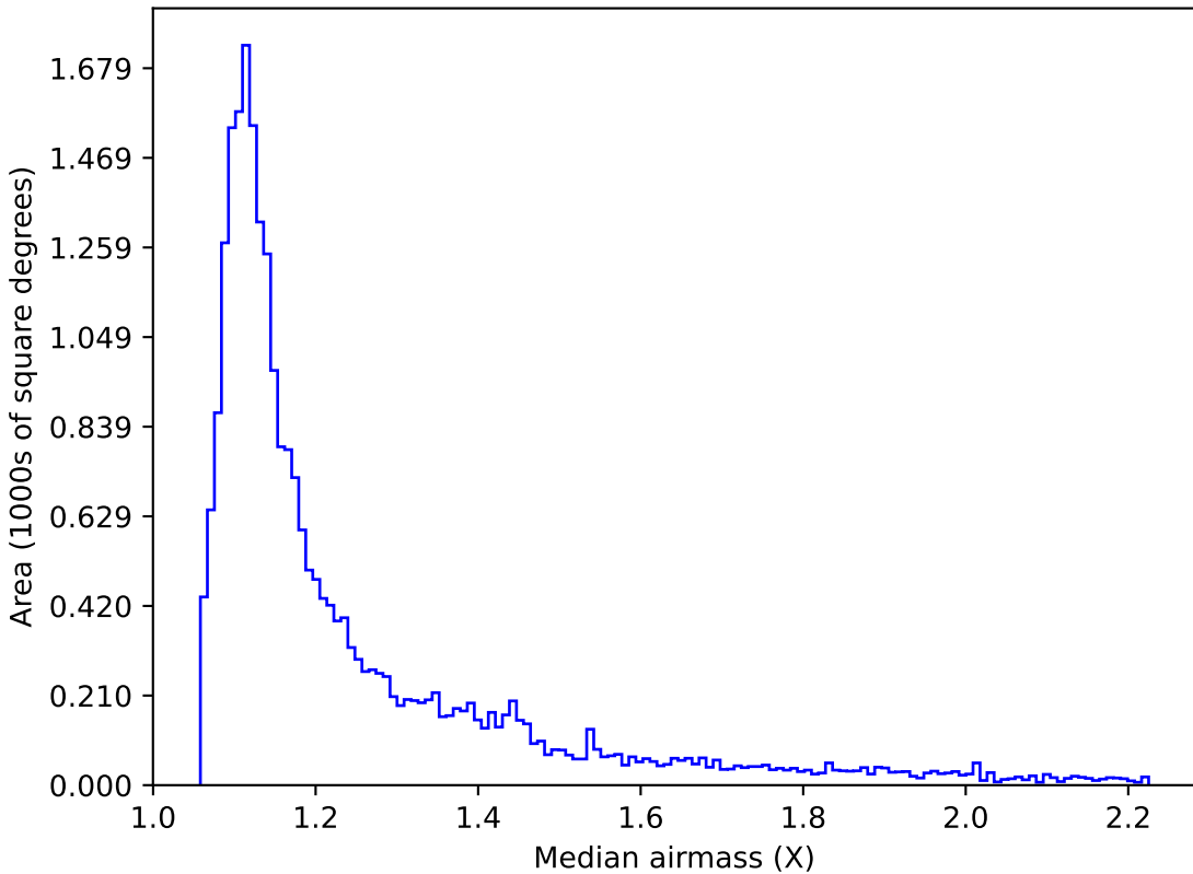
extra_ss_neo2_v3.4_10yrs Yr 1 i band: Median airmass
