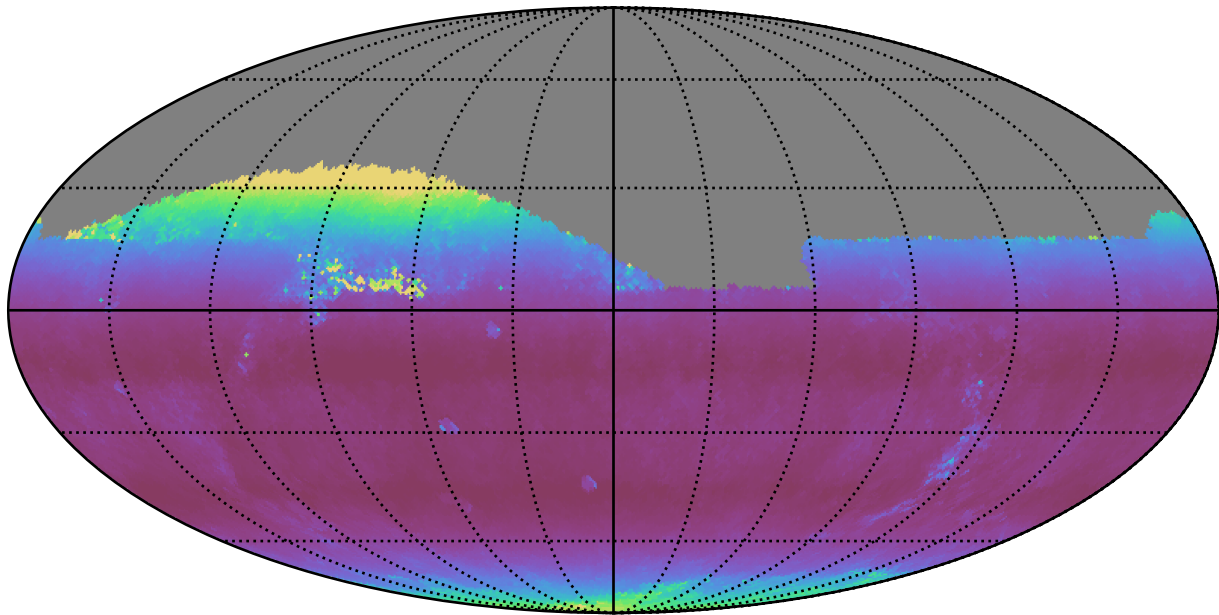
extra_ss_neo2_v3.4_10yrs Yr 1 all bands: Median airmass
