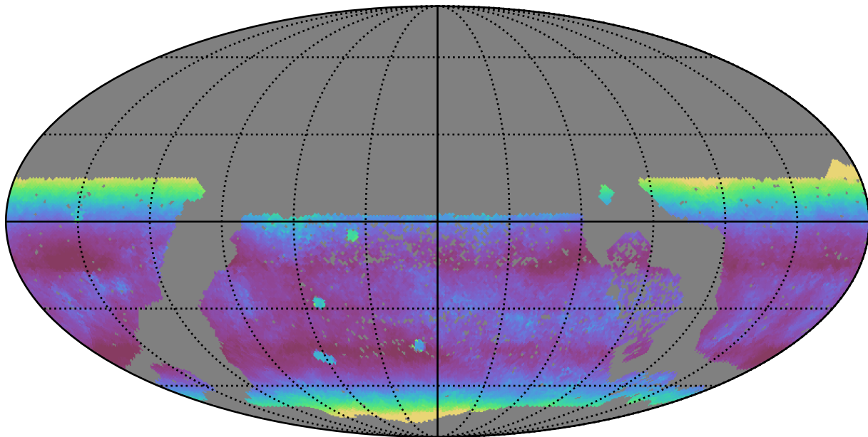
extra_ss_neo2_v3.4_10yrs WFD z band: Median airmass
