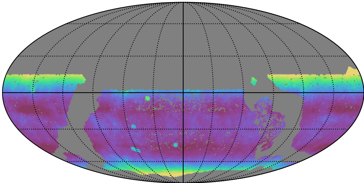
extra_ss_neo2_v3.4_10yrs WFD y band: Median airmass
