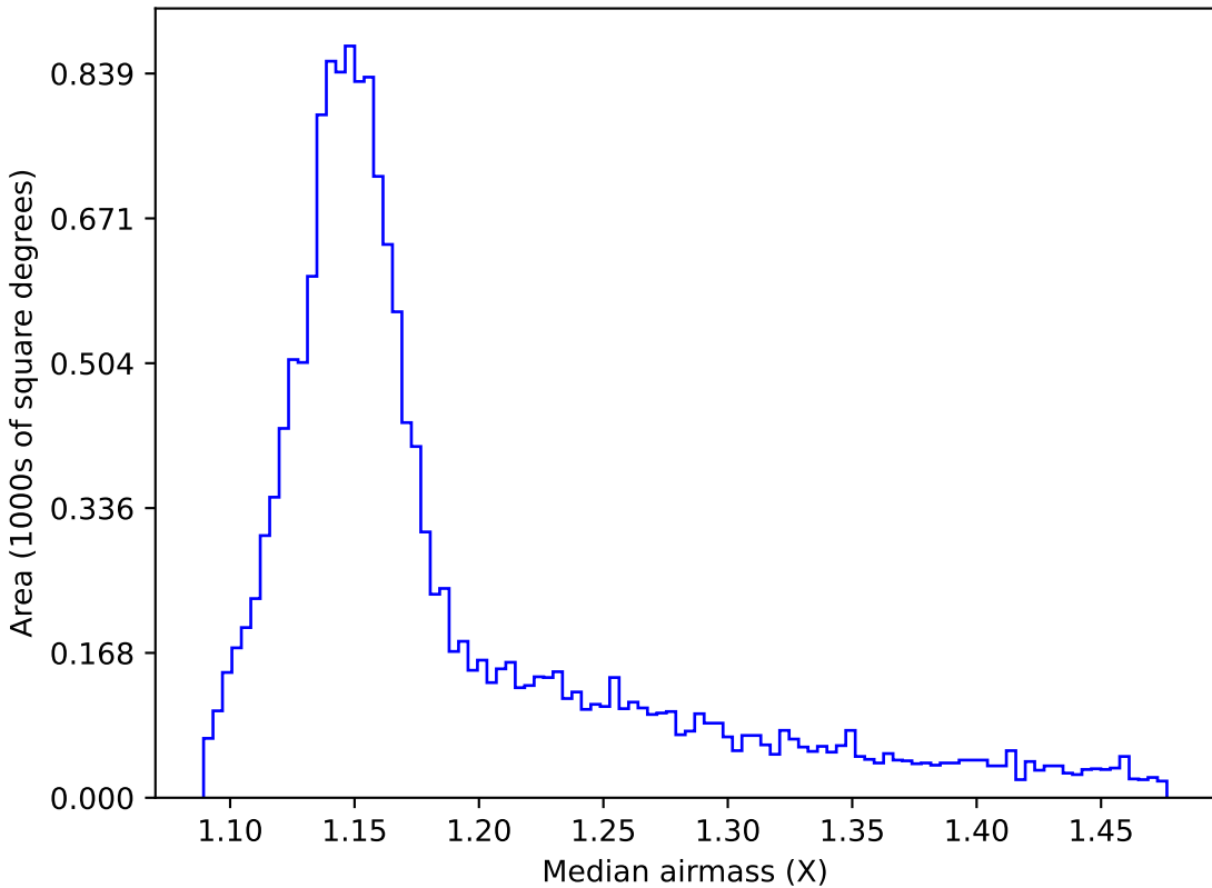
extra_ss_neo2_v3.4_10yrs WFD y band: Median airmass
