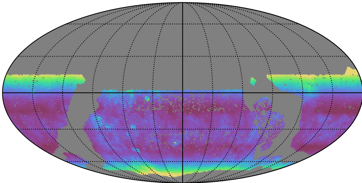
extra_ss_neo2_v3.4_10yrs WFD u band: Median airmass
