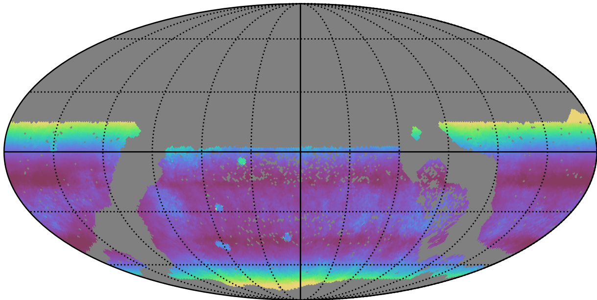
extra_ss_neo2_v3.4_10yrs WFD r band: Median airmass
