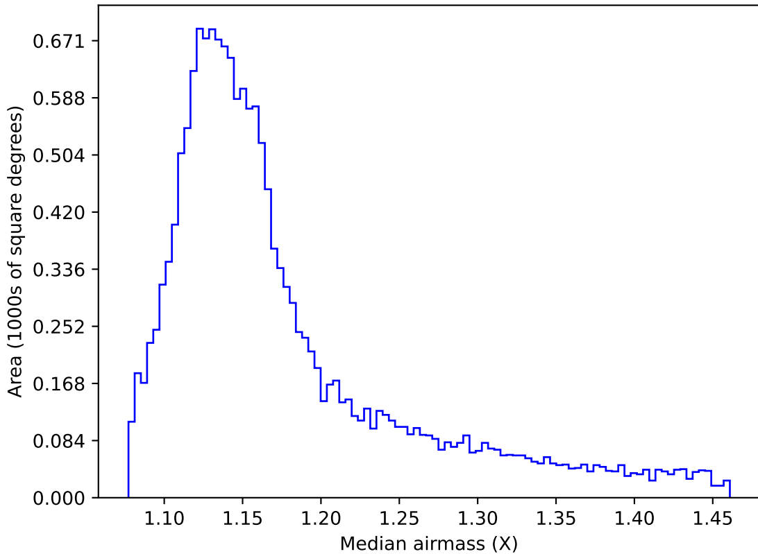
extra_ss_neo2_v3.4_10yrs WFD r band: Median airmass
