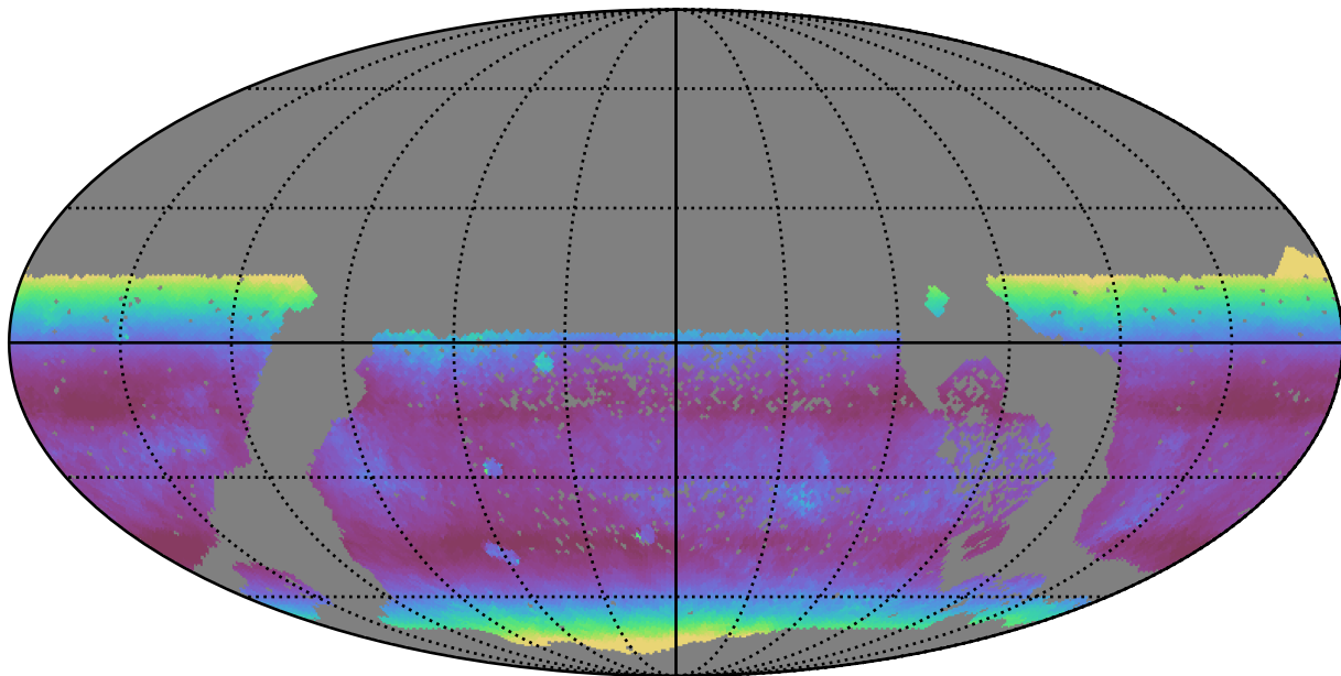
extra_ss_neo2_v3.4_10yrs WFD i band: Median airmass
