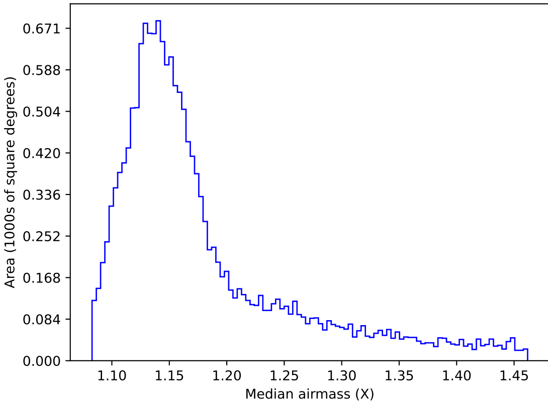
extra_ss_neo2_v3.4_10yrs WFD i band: Median airmass
