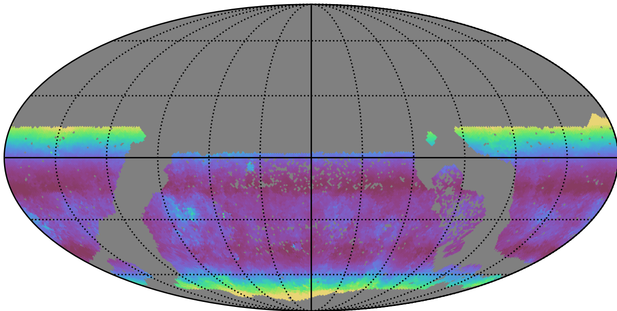
extra_ss_neo2_v3.4_10yrs WFD g band: Median airmass
