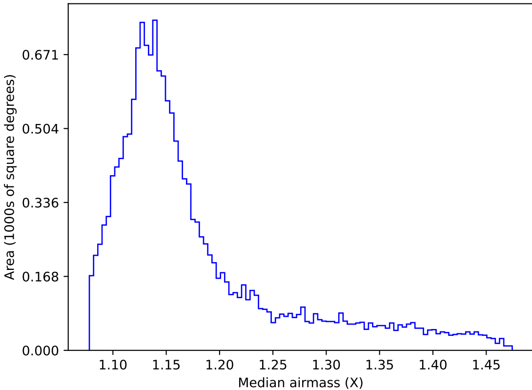
extra_ss_neo2_v3.4_10yrs WFD g band: Median airmass
