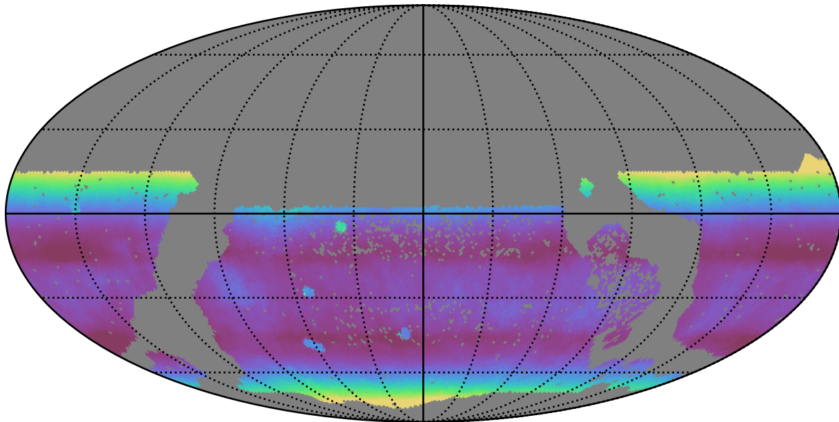
extra_ss_neo2_v3.4_10yrs WFD all bands: Median airmass
