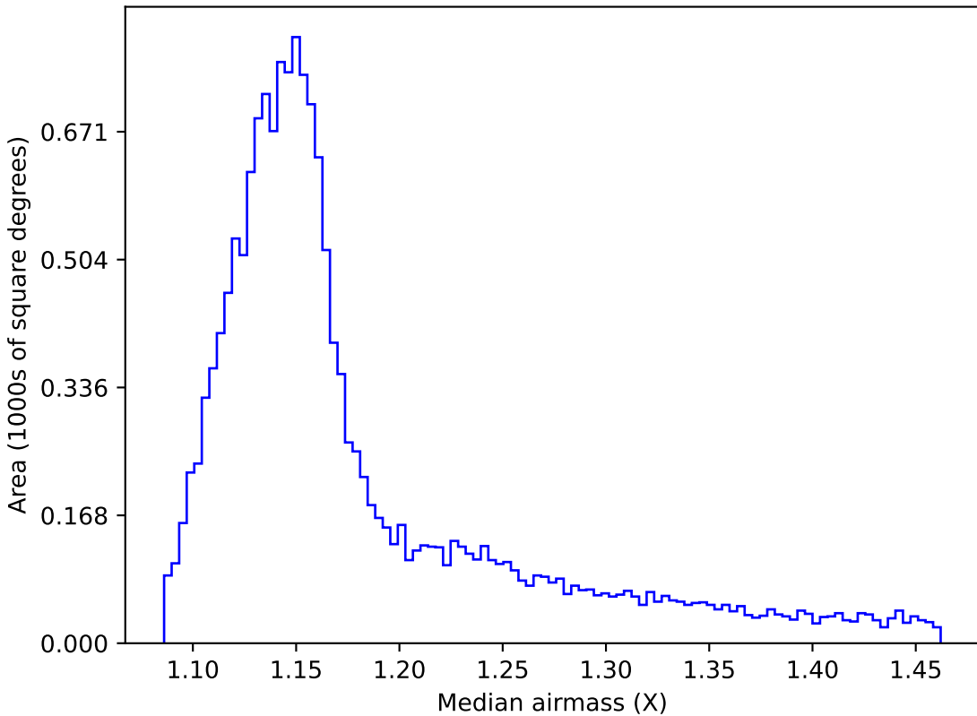
extra_ss_neo2_v3.4_10yrs WFD all bands: Median airmass
