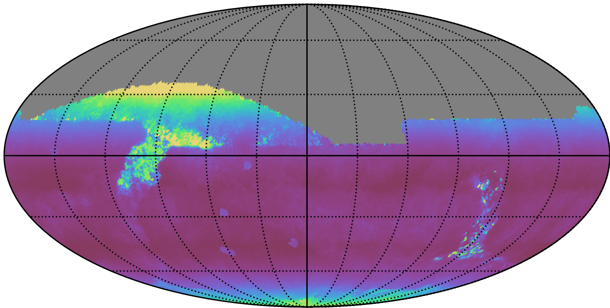
extra_ss_neo2_v3.4_10yrs All sky z band: Median airmass
