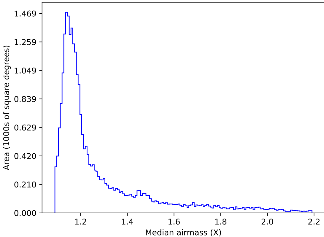
extra_ss_neo2_v3.4_10yrs All sky z band: Median airmass
