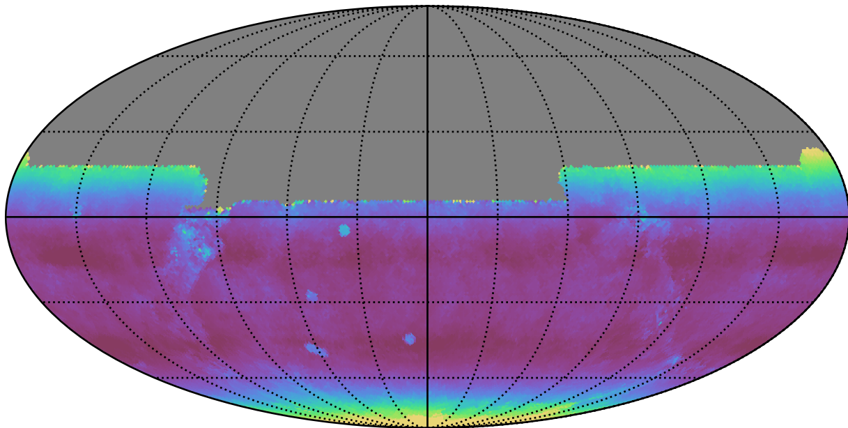
extra_ss_neo2_v3.4_10yrs All sky y band: Median airmass
