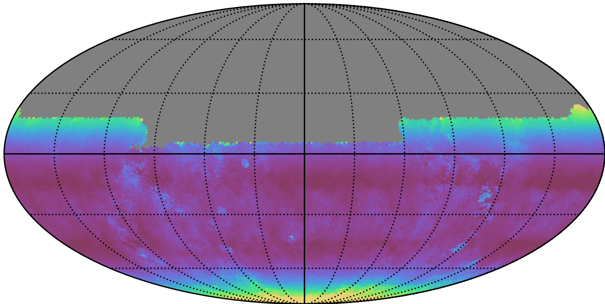
extra_ss_neo2_v3.4_10yrs All sky u band: Median airmass
