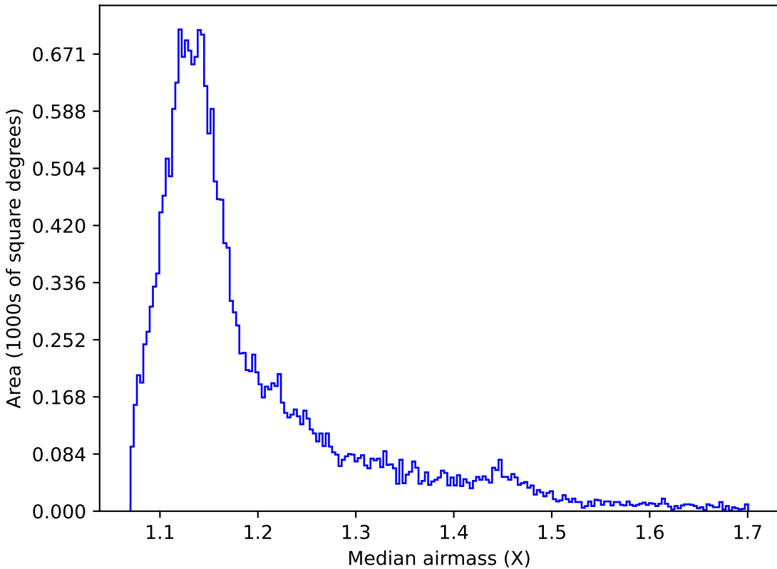
extra_ss_neo2_v3.4_10yrs All sky u band: Median airmass
