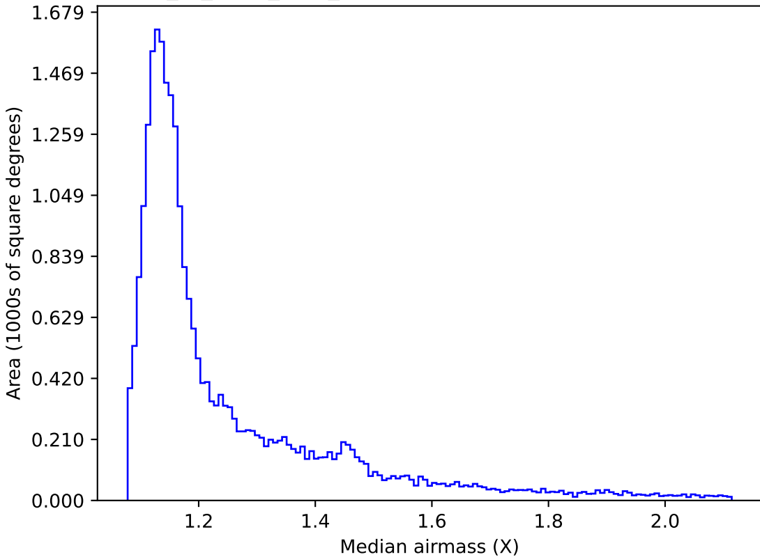
extra_ss_neo2_v3.4_10yrs All sky r band: Median airmass
