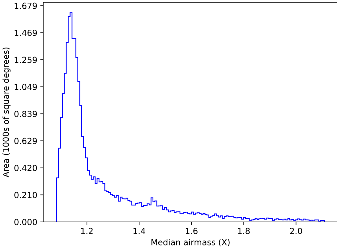
extra_ss_neo2_v3.4_10yrs All sky i band: Median airmass
