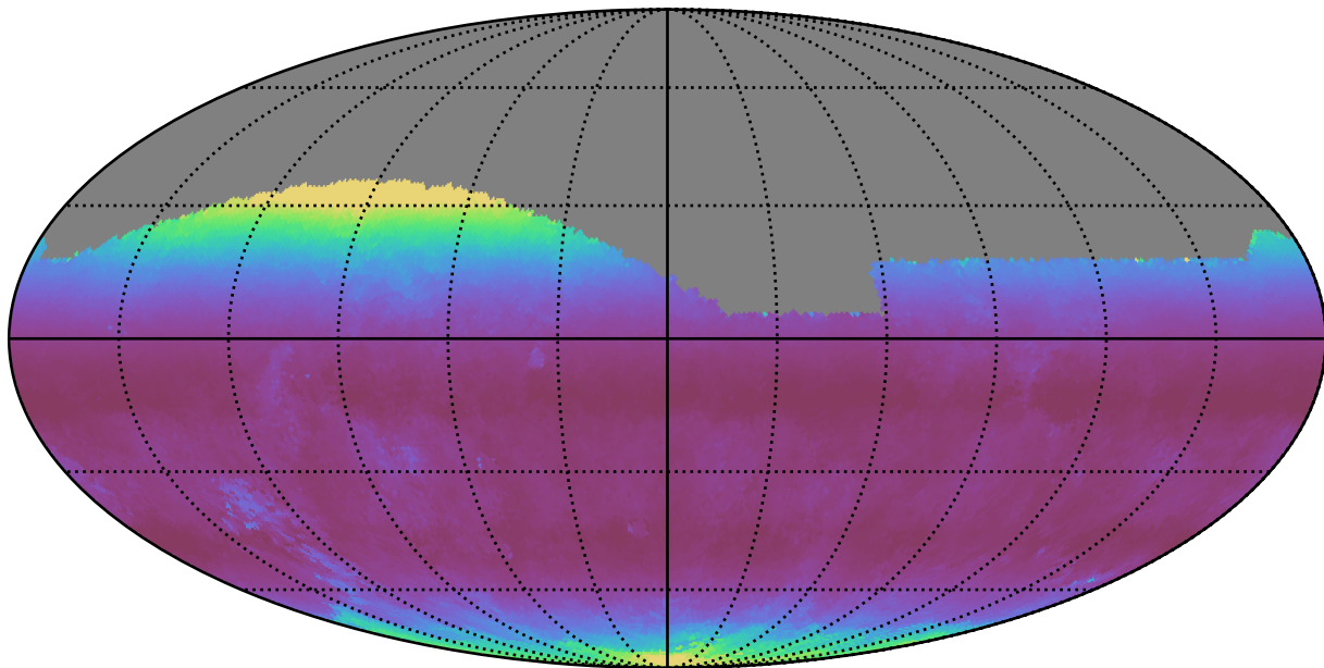
extra_ss_neo2_v3.4_10yrs All sky g band: Median airmass
