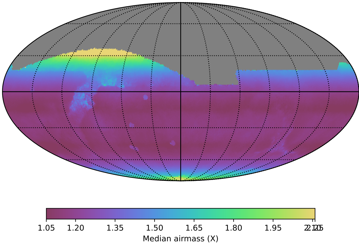
extra_ss_neo2_v3.4_10yrs All sky all bands: Median airmass
