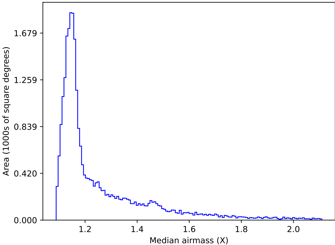
extra_ss_neo2_v3.4_10yrs All sky all bands: Median airmass
