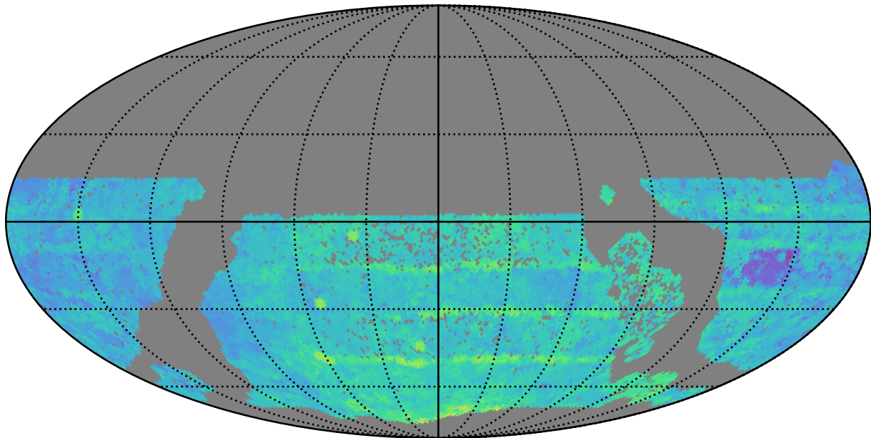
extra_ss_neo2_v3.4_10yrs WFD z band: Median Season Length
