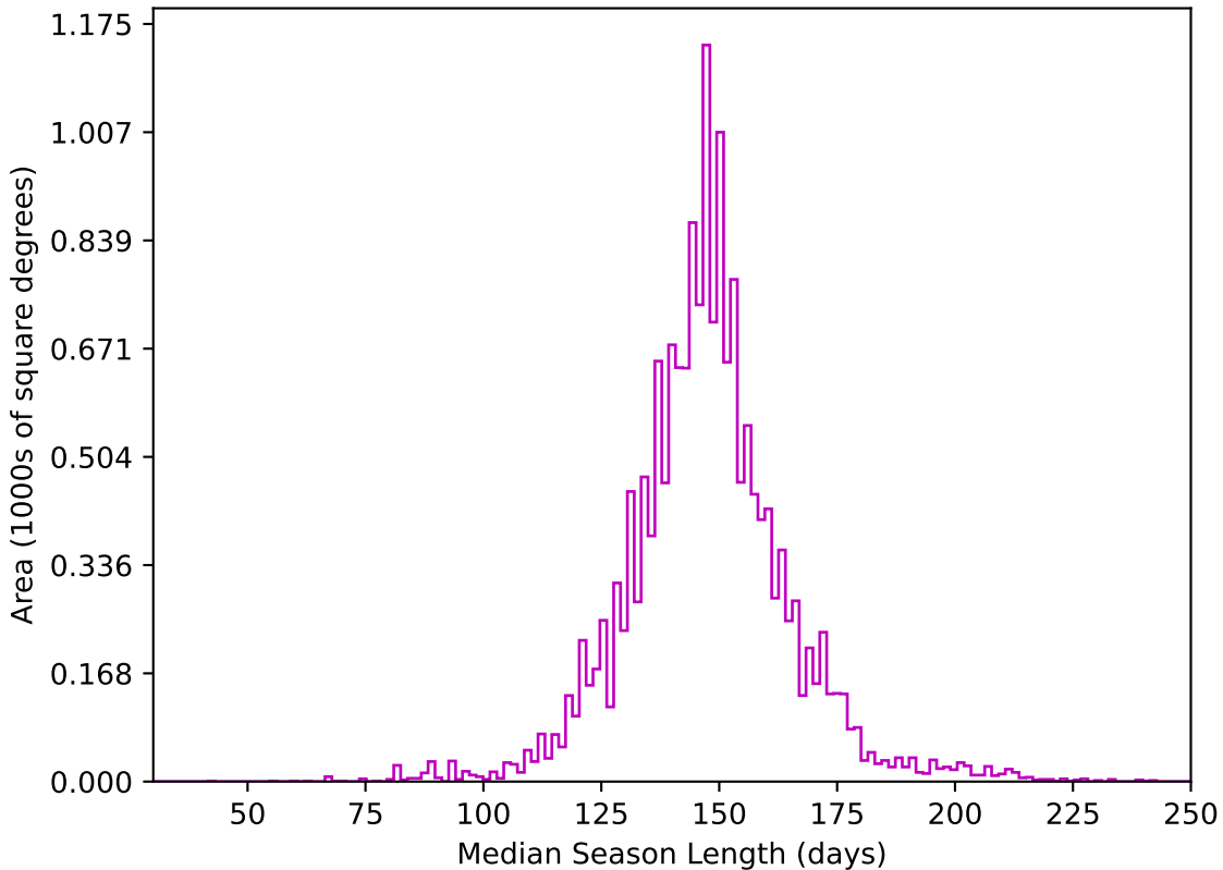
extra_ss_neo2_v3.4_10yrs WFD z band: Median Season Length
