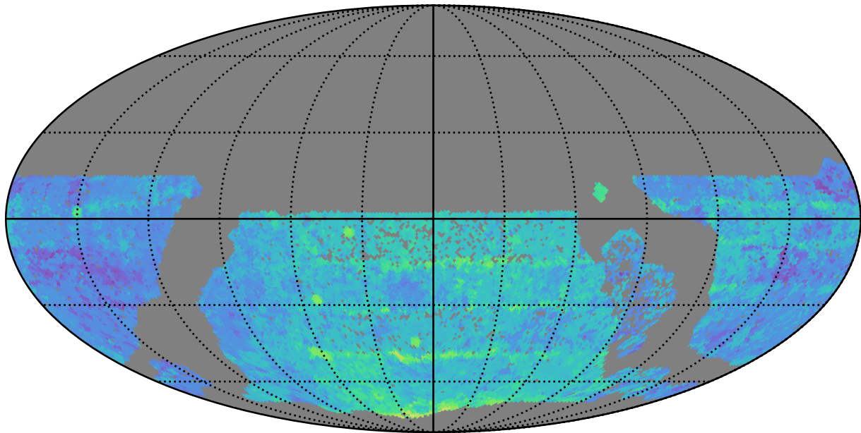
extra_ss_neo2_v3.4_10yrs WFD y band: Median Season Length
