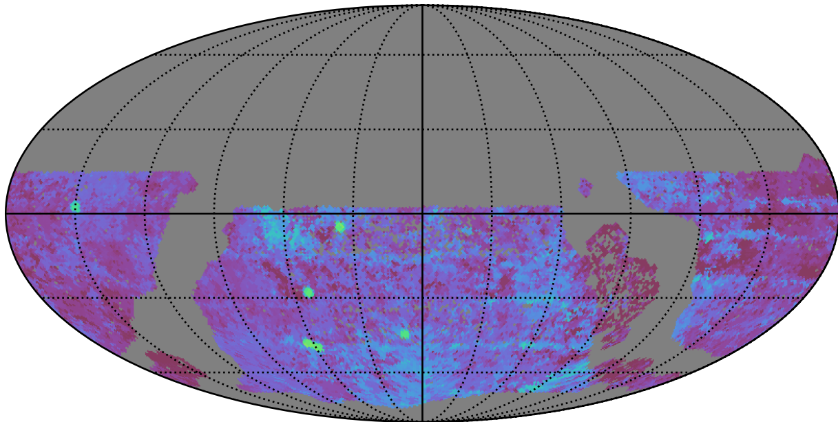
extra_ss_neo2_v3.4_10yrs WFD u band: Median Season Length
