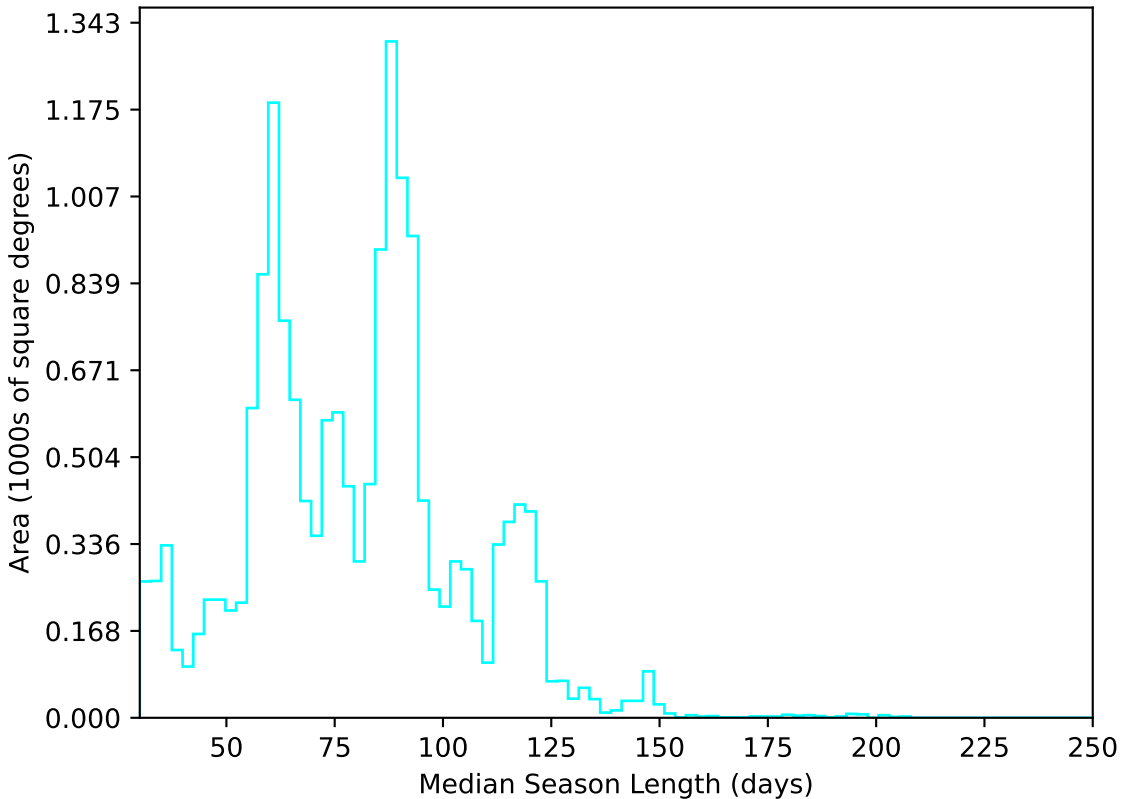
extra_ss_neo2_v3.4_10yrs WFD u band: Median Season Length
