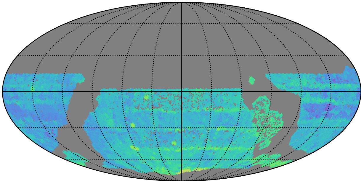
extra_ss_neo2_v3.4_10yrs WFD r band: Median Season Length
