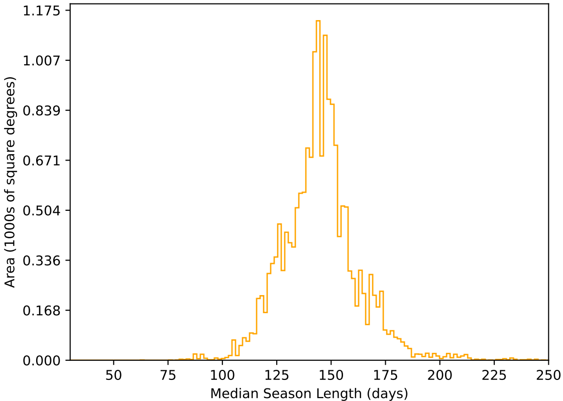
extra_ss_neo2_v3.4_10yrs WFD r band: Median Season Length
