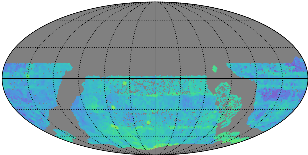
extra_ss_neo2_v3.4_10yrs WFD i band: Median Season Length
