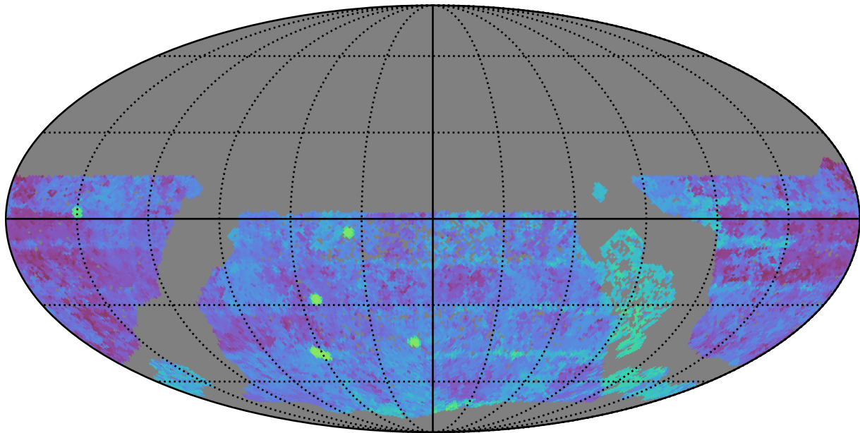
extra_ss_neo2_v3.4_10yrs WFD g band: Median Season Length
