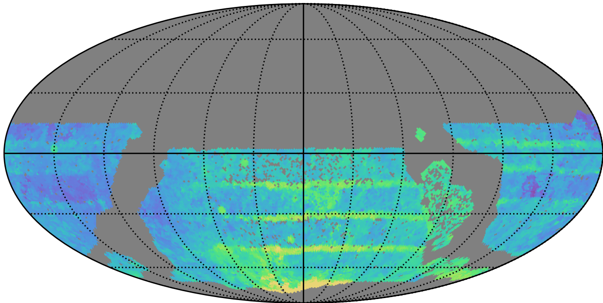
extra_ss_neo2_v3.4_10yrs WFD all bands: Median Season Length
