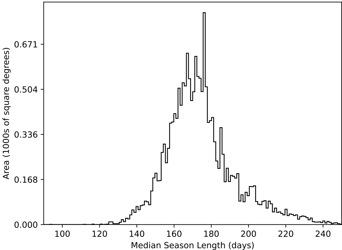
extra_ss_neo2_v3.4_10yrs WFD all bands: Median Season Length
