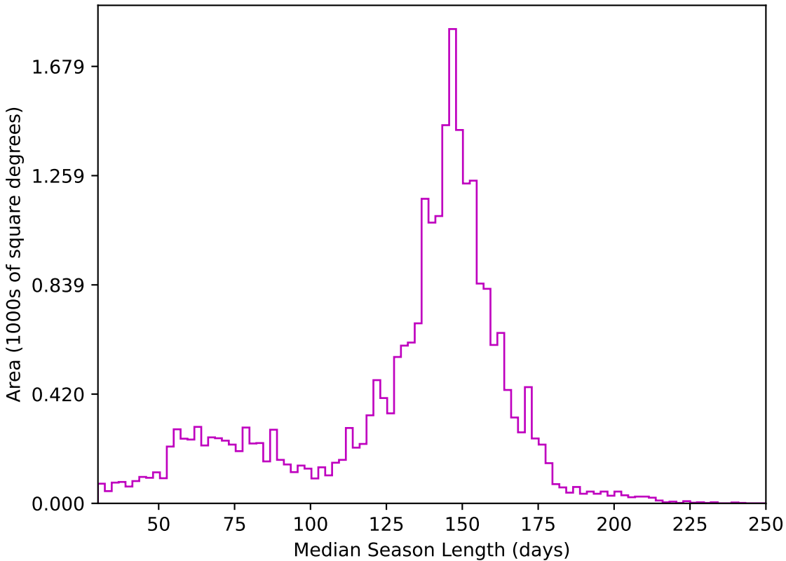
extra_ss_neo2_v3.4_10yrs All sky z band: Median Season Length
