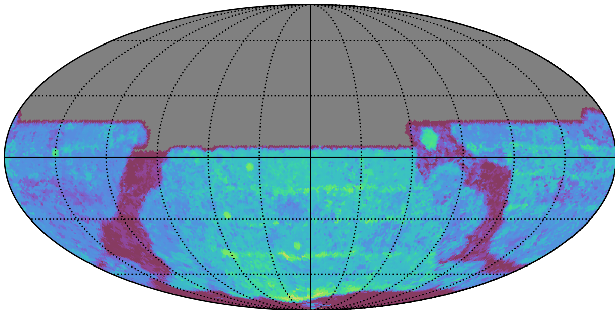
extra_ss_neo2_v3.4_10yrs All sky y band: Median Season Length
