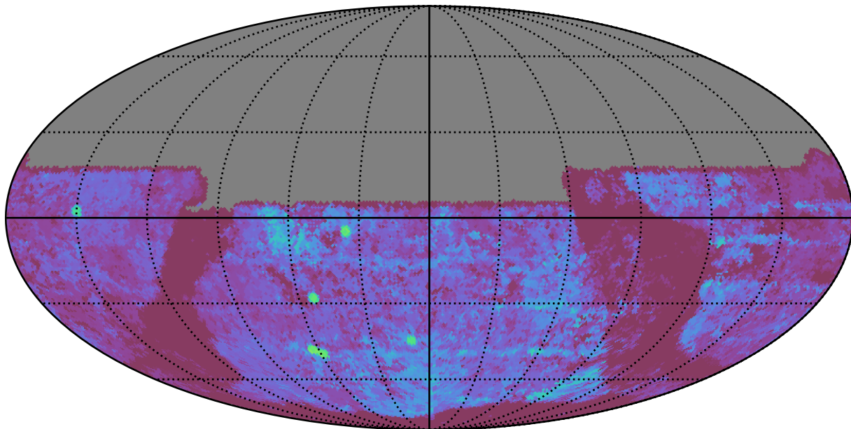
extra_ss_neo2_v3.4_10yrs All sky u band: Median Season Length
