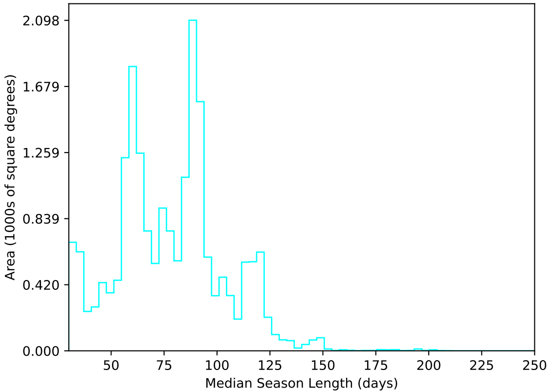
extra_ss_neo2_v3.4_10yrs All sky u band: Median Season Length
