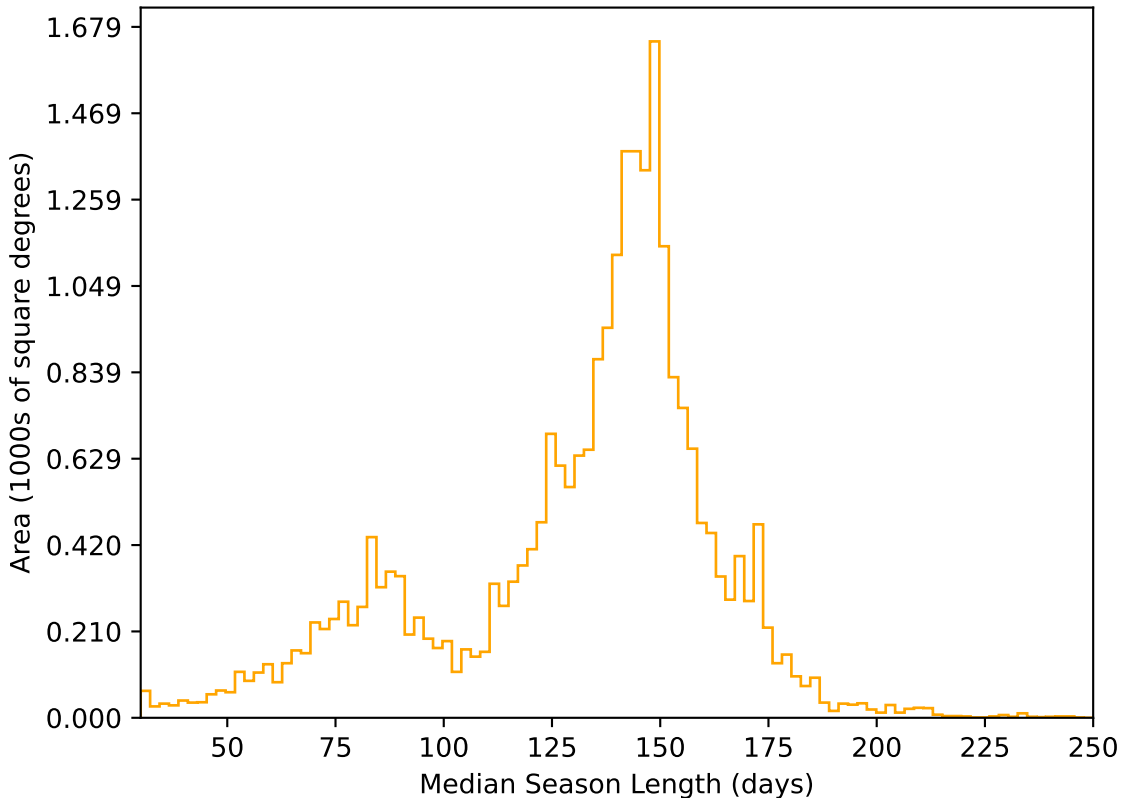
extra_ss_neo2_v3.4_10yrs All sky r band: Median Season Length
