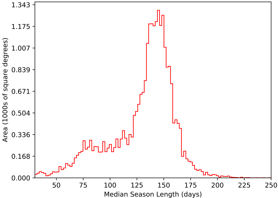
extra_ss_neo2_v3.4_10yrs All sky i band: Median Season Length
