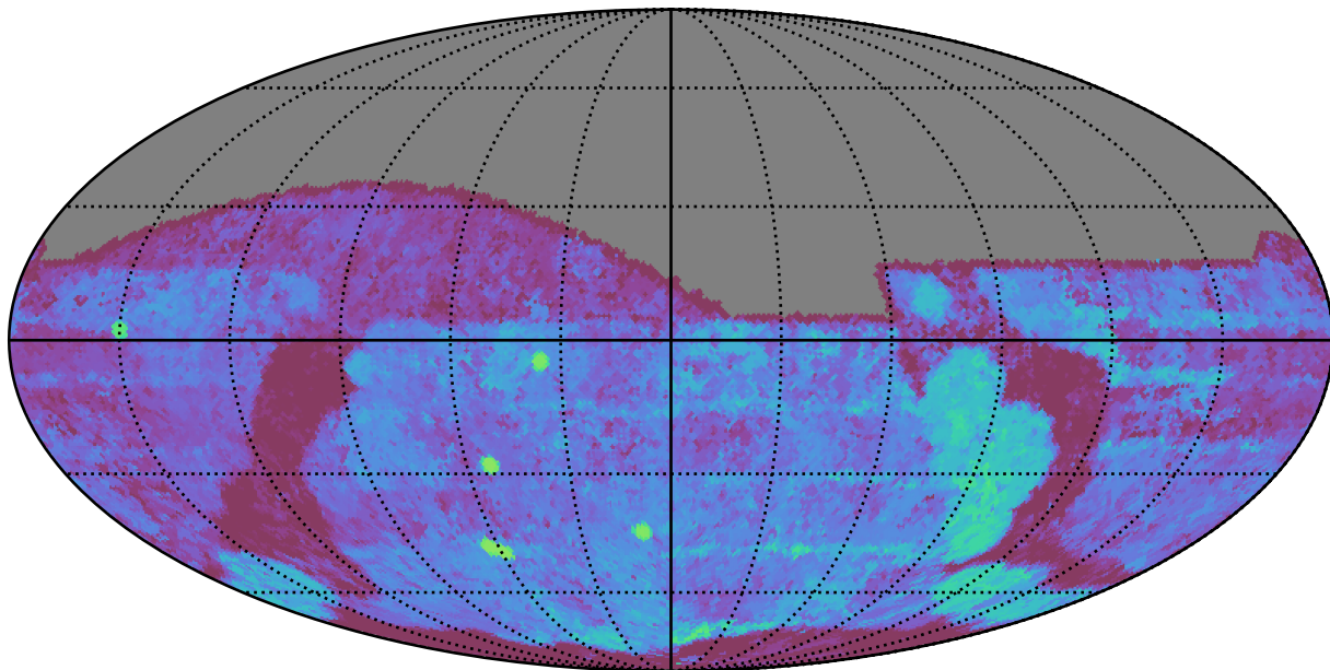
extra_ss_neo2_v3.4_10yrs All sky g band: Median Season Length
