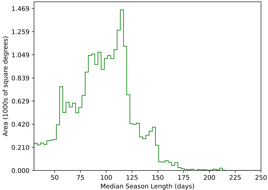
extra_ss_neo2_v3.4_10yrs All sky g band: Median Season Length
