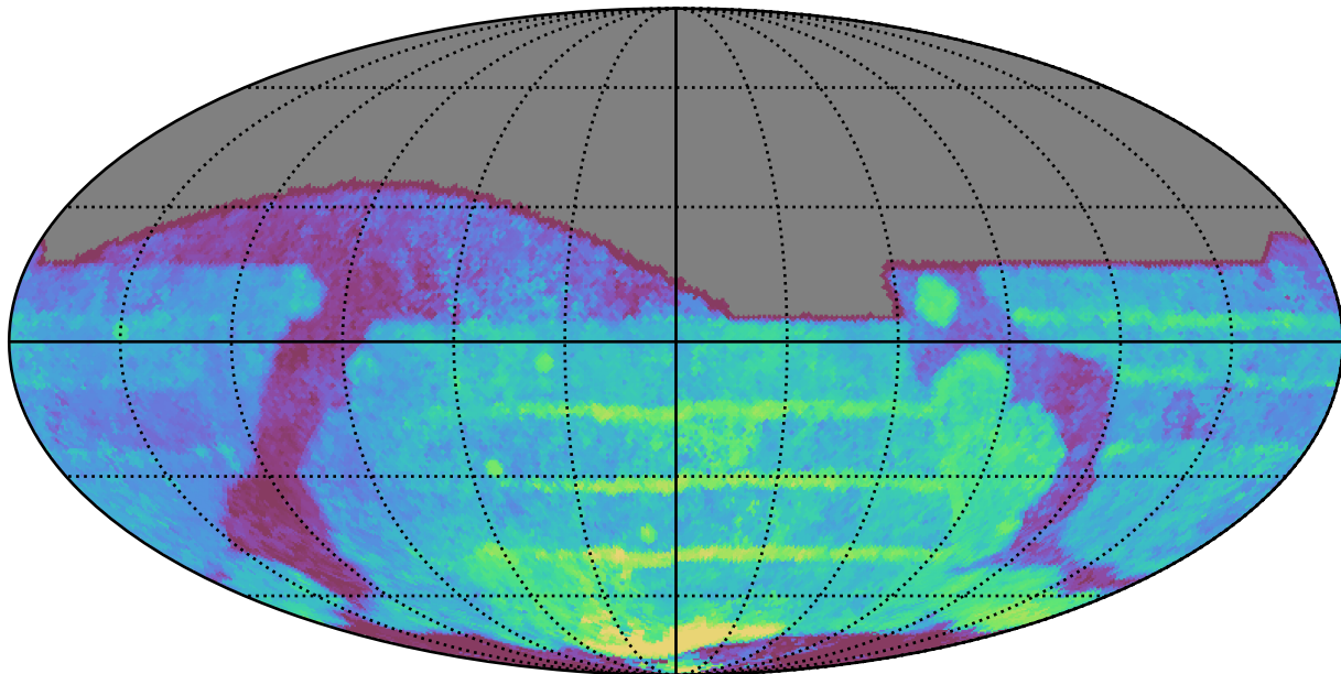
extra_ss_neo2_v3.4_10yrs All sky all bands: Median Season Length
