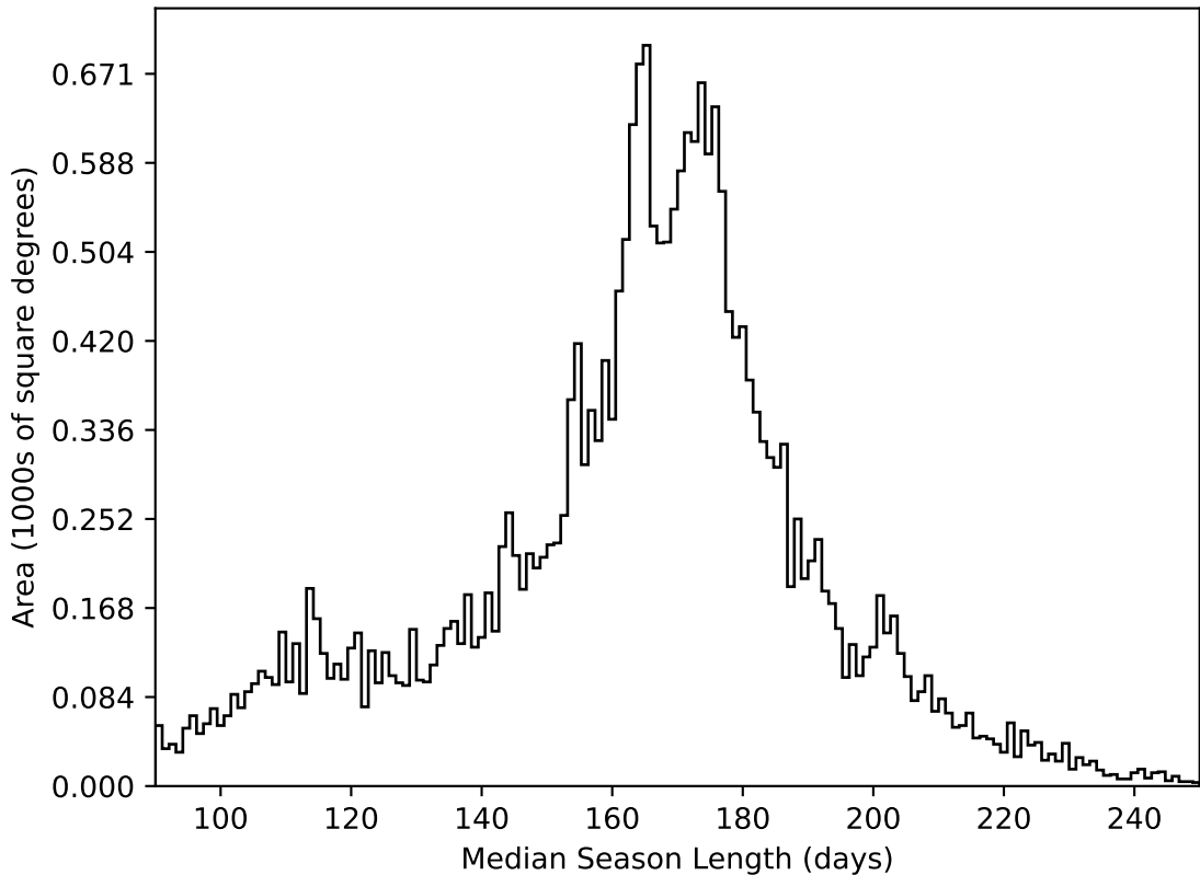
extra_ss_neo2_v3.4_10yrs All sky all bands: Median Season Length
