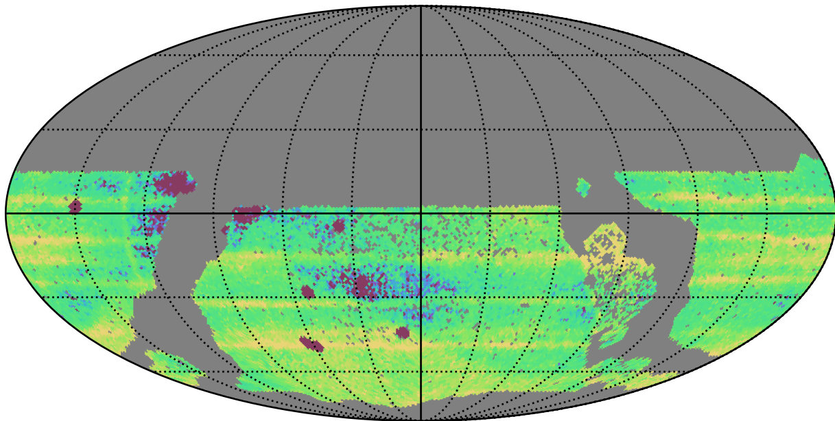
extra_ss_neo2_v3.4_10yrs WFD: Median Intra-Night Gap
